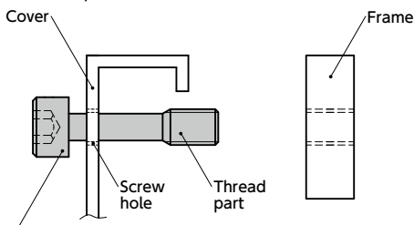
SSC-RY Hex socket head cap captive screw
