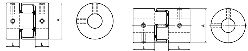
Set Screw Type MJC MJC - K
